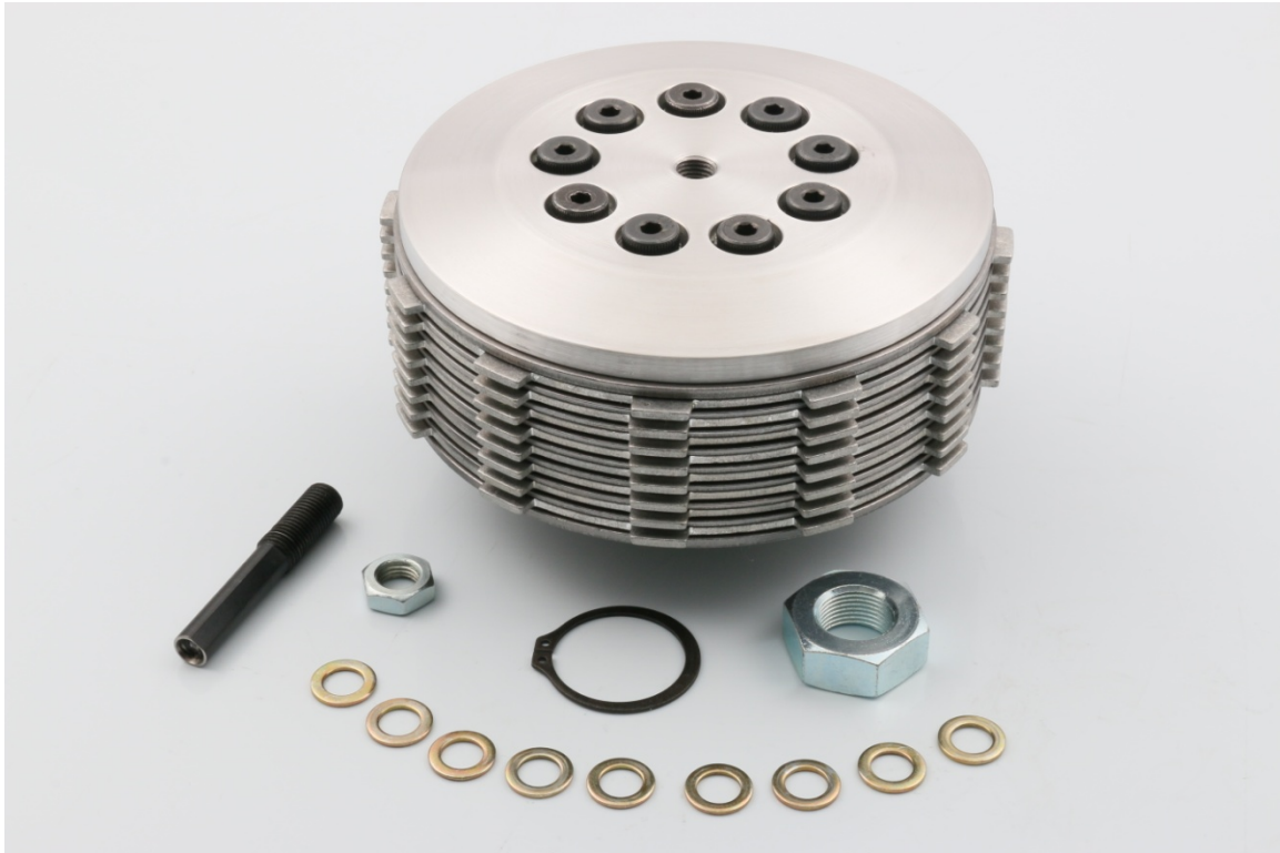
Top picture CC-122-CSPP, Competitor Clutch Complete. Fits 2011-2016 Big Twins. W/ cable clutch
